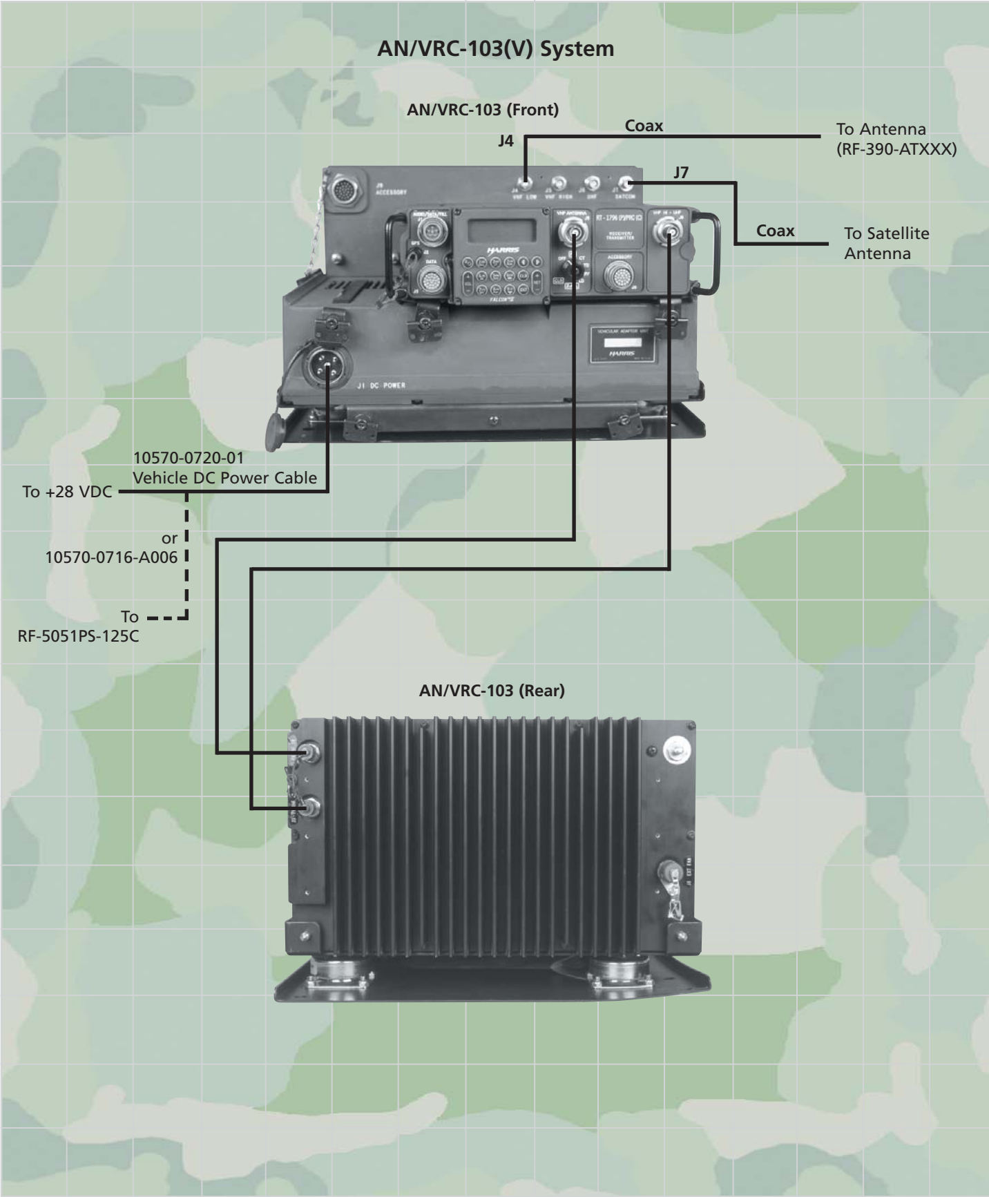
AN/VRC-103 System Interconnect Diagram
